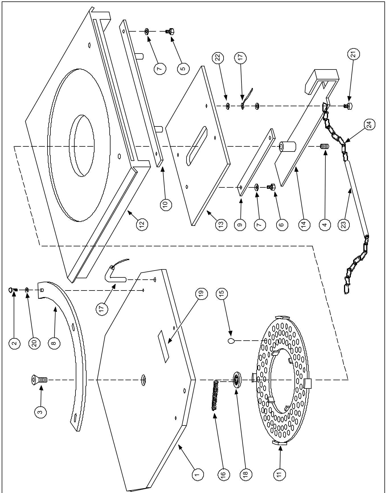
25-24-1/25-71-1 TRUCK TURNING ANGLE GAUGE REFER TO OPPOSITE SIDE FOR PARTS DESCRIPTION LISTING
